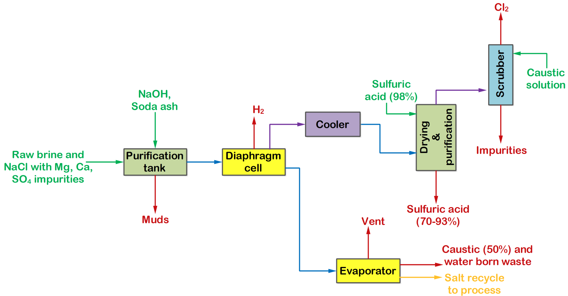
Figure: Manufacture of chlorine by diaphragm cell process
